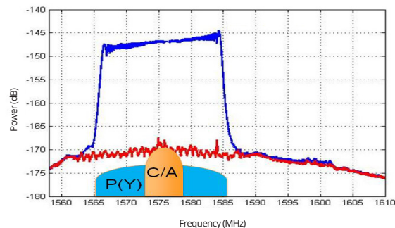
GPS L1 signal contaminated with a chirp jammer signal: before (blue) and after (red) activation of WIMU also shown on page 6
