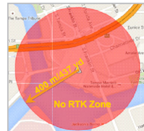
Figure 13 – 10 mW Chirp jammer without mitigation
